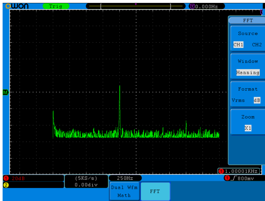
Fig.5-11 Hanning window
