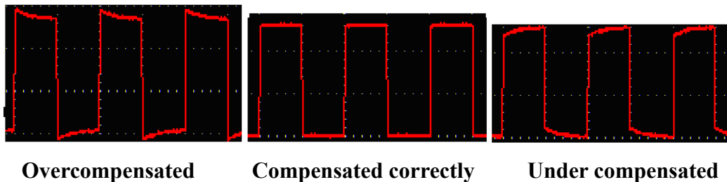
Fig. 4-8 Displayed Waveforms of the Probe Compensation
